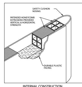
INTERNAL CONSTRUCTION
